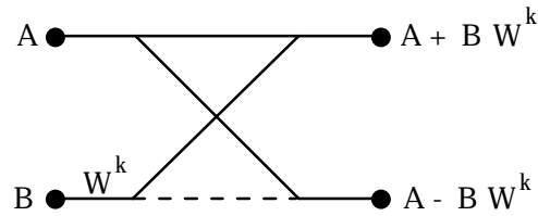
Figure 1: FFT Butterfly. The dashed line indicates negation.
